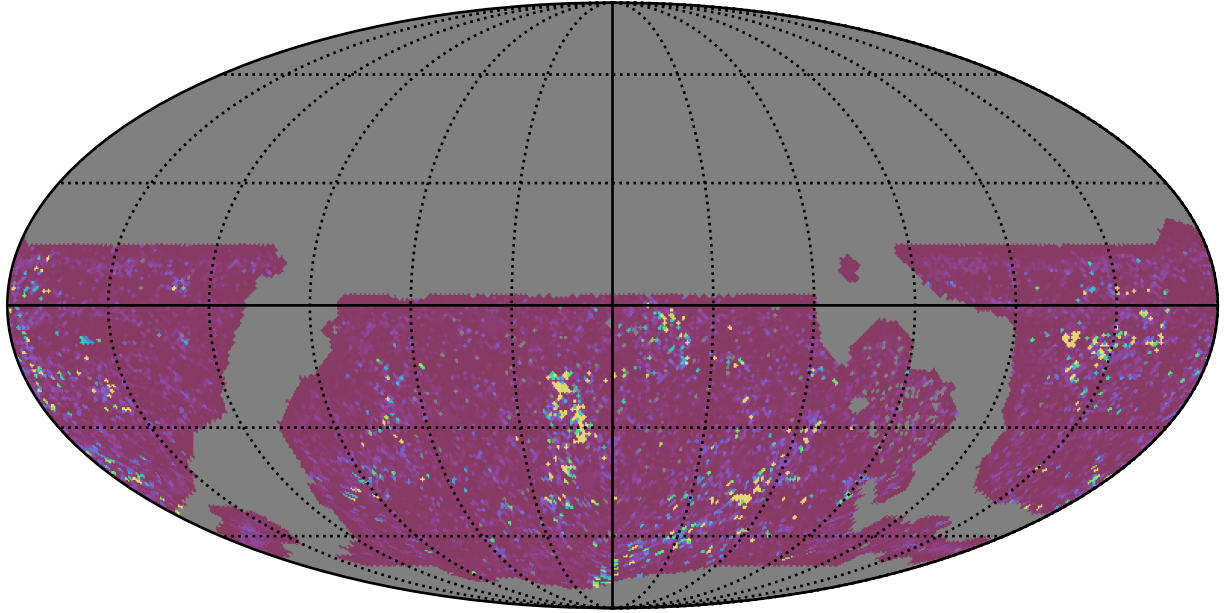
roll_uniform_early_half_mjdp0_v3.4_10yrs WFD g band: 75th Percentile Intranight Timespan
