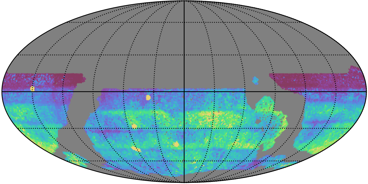
roll_uniform_early_half_mjdp0_v3.4_10yrs WFD all bands: 75th Percentile Intranight Timespan
