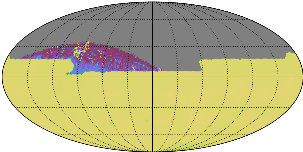
roll_uniform_early_half_mjdp0_v3.4_10yrs All sky zy bands: 75th Percentile Intranight Timespan
