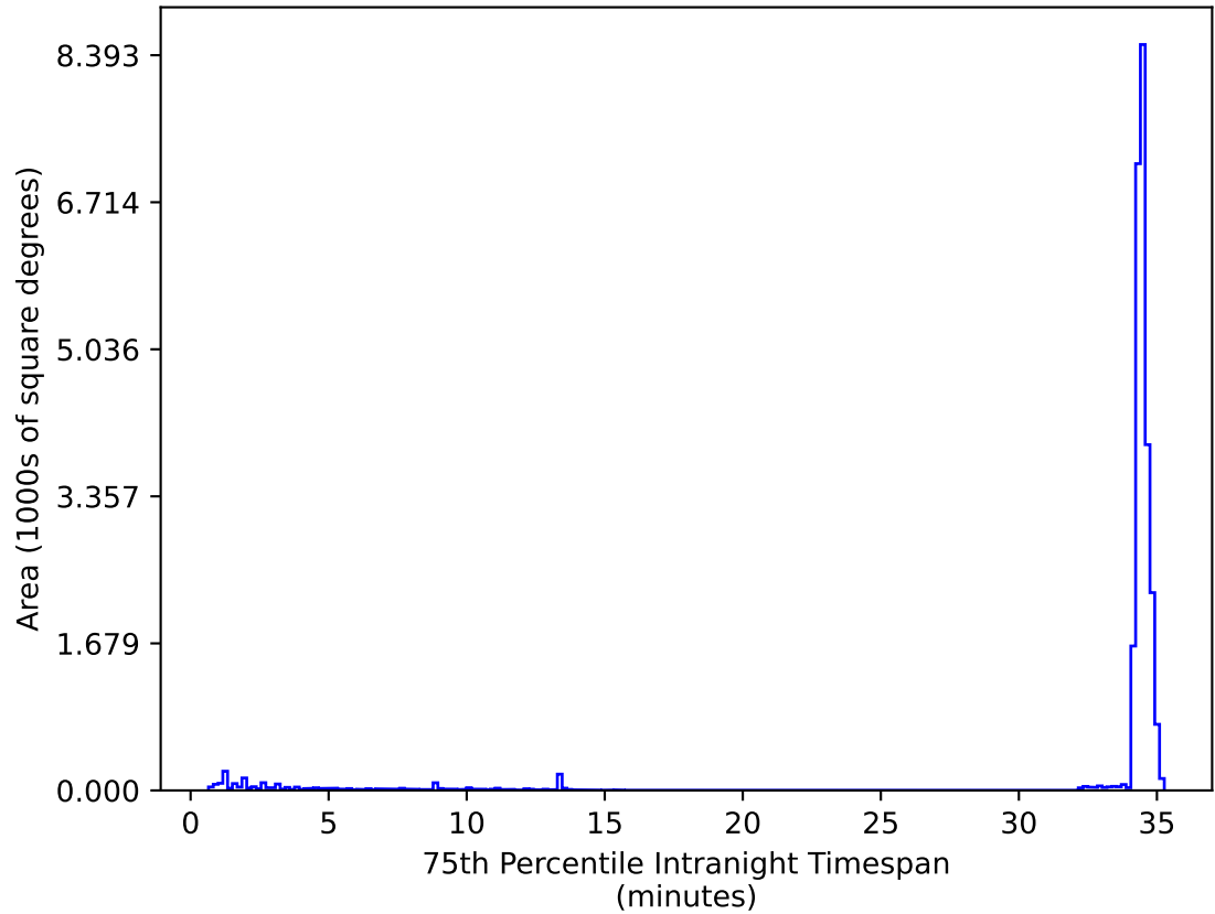
roll_uniform_early_half_mjdp0_v3.4_10yrs All sky zy bands: 75th Percentile Intranight Timespan
