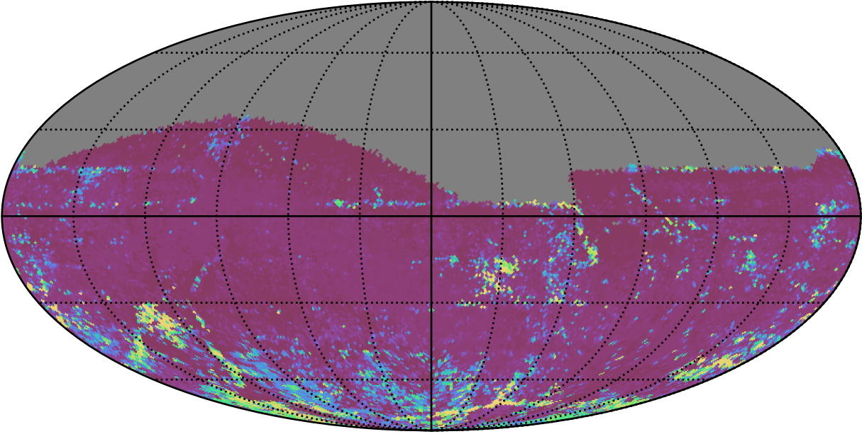
roll_uniform_early_half_mjdp0_v3.4_10yrs All sky z band: 75th Percentile Intranight Timespan
