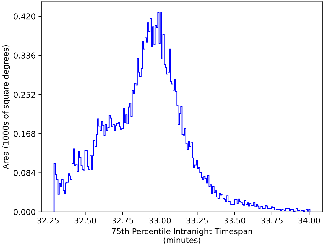
roll_uniform_early_half_mjdp0_v3.4_10yrs All sky y band: 75th Percentile Intranight Timespan
