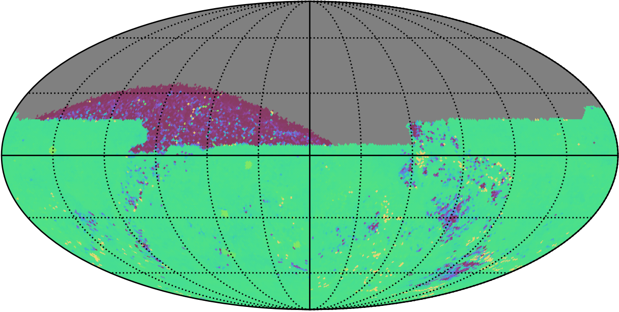
roll_uniform_early_half_mjdp0_v3.4_10yrs All sky ug bands: 75th Percentile Intranight Timespan
