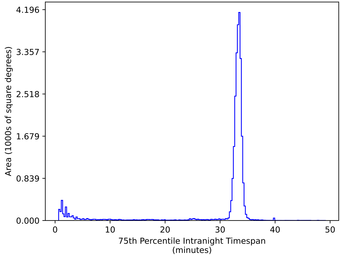
roll_uniform_early_half_mjdp0_v3.4_10yrs All sky ug bands: 75th Percentile Intranight Timespan
