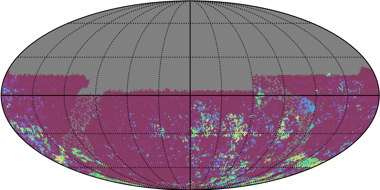
roll_uniform_early_half_mjdp0_v3.4_10yrs All sky u band: 75th Percentile Intranight Timespan
