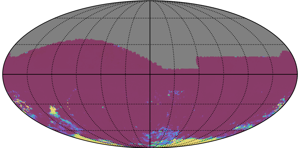
roll_uniform_early_half_mjdp0_v3.4_10yrs All sky ri bands: 75th Percentile Intranight Timespan
