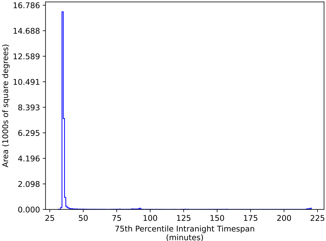
roll_uniform_early_half_mjdp0_v3.4_10yrs All sky ri bands: 75th Percentile Intranight Timespan
