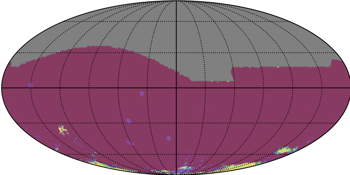
roll_uniform_early_half_mjdp0_v3.4_10yrs All sky iz bands: 75th Percentile Intranight Timespan
