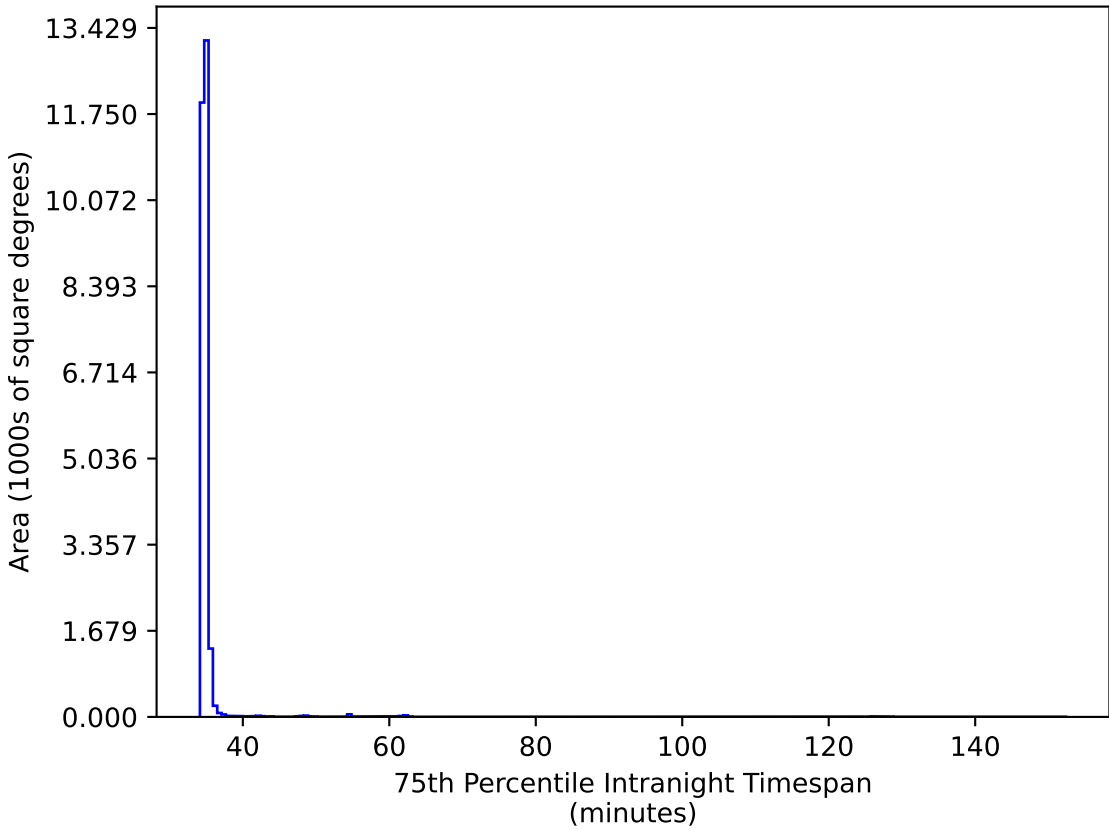
roll_uniform_early_half_mjdp0_v3.4_10yrs All sky iz bands: 75th Percentile Intranight Timespan
