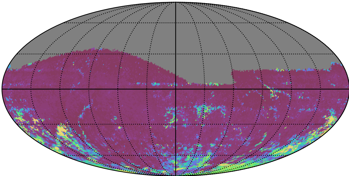
roll_uniform_early_half_mjdp0_v3.4_10yrs All sky i band: 75th Percentile Intranight Timespan
