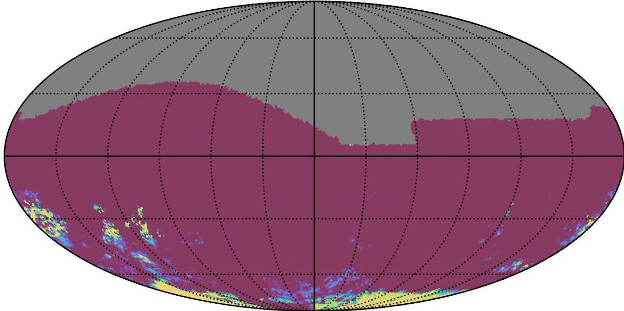
roll_uniform_early_half_mjdp0_v3.4_10yrs All sky gr bands: 75th Percentile Intranight Timespan
