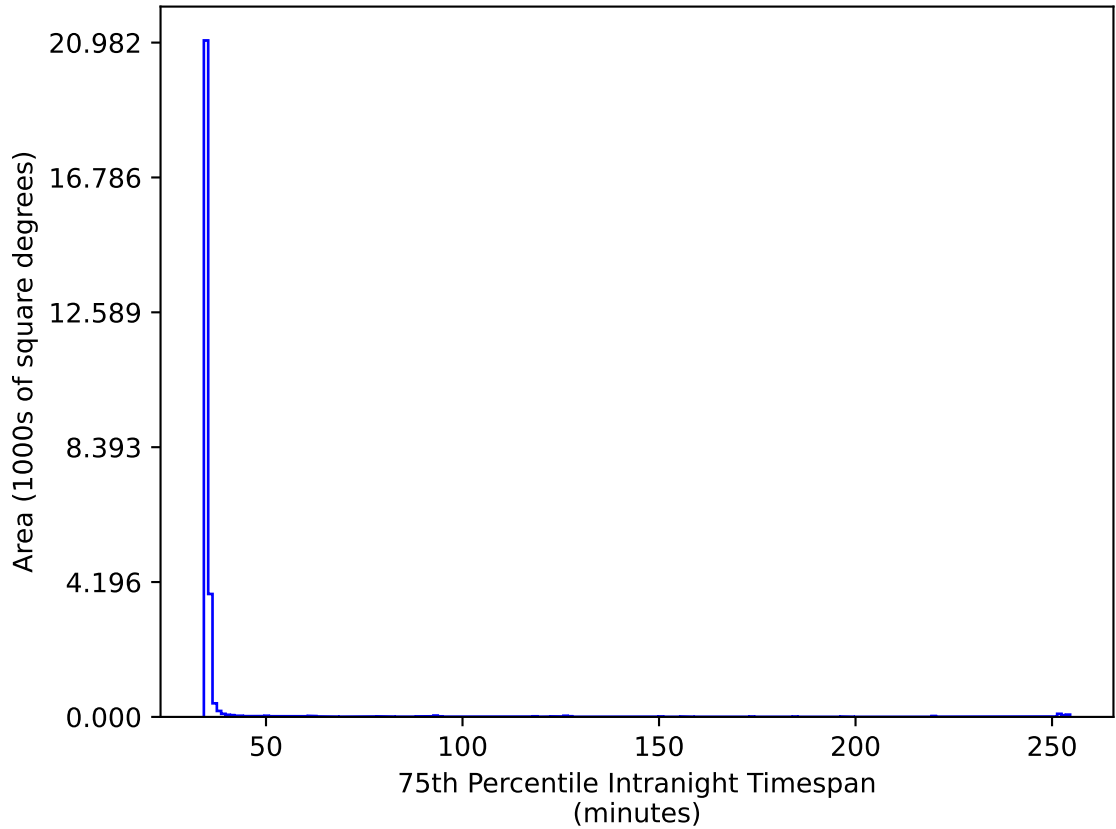
roll_uniform_early_half_mjdp0_v3.4_10yrs All sky gr bands: 75th Percentile Intranight Timespan
