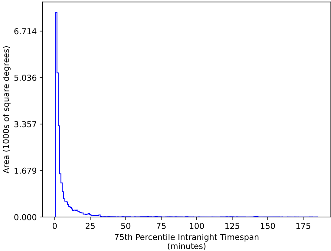
roll_uniform_early_half_mjdp0_v3.4_10yrs All sky g band: 75th Percentile Intranight Timespan
