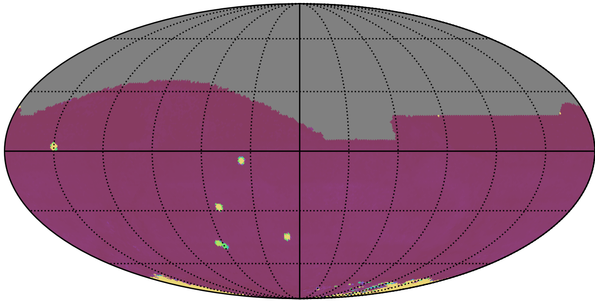
roll_uniform_early_half_mjdp0_v3.4_10yrs All sky all bands: 75th Percentile Intranight Timespan
