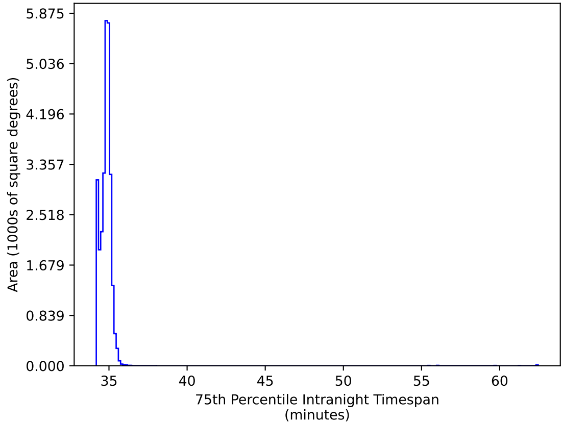
roll_uniform_early_half_mjdp0_v3.4_10yrs All sky all bands: 75th Percentile Intranight Timespan
