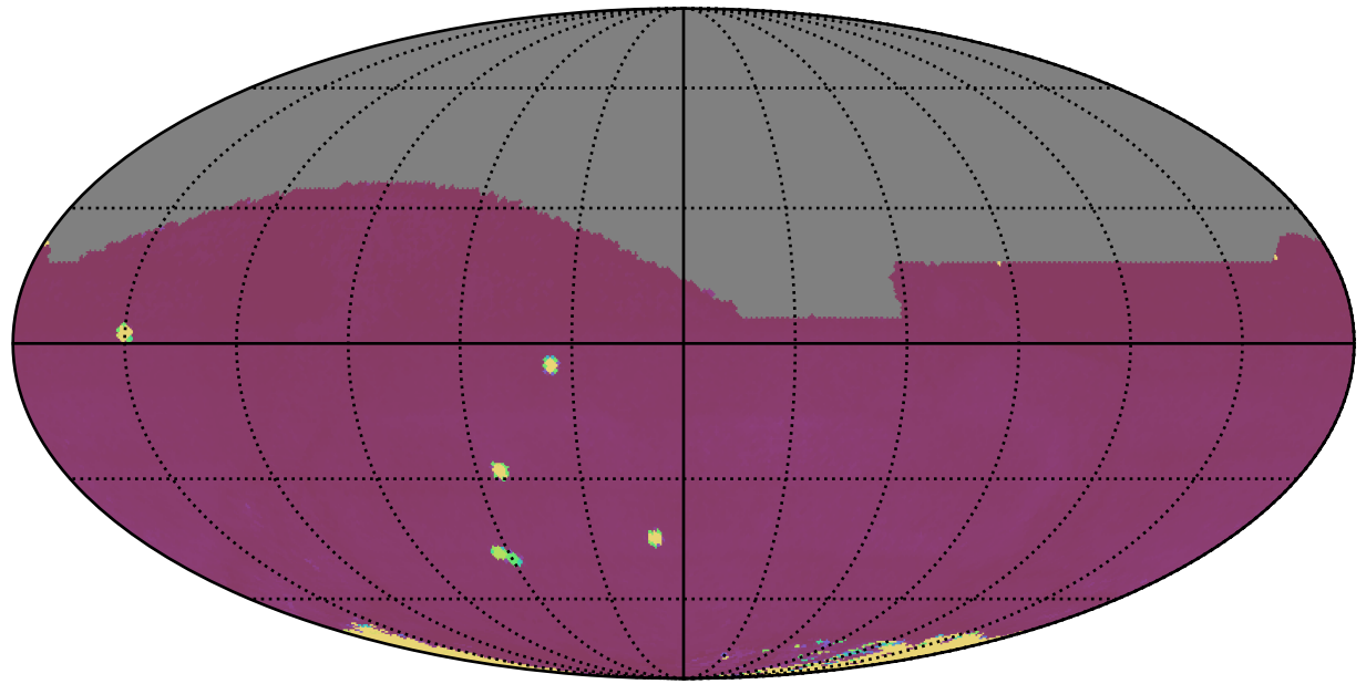
roll_uniform_early_half_mjdp0_v3.4_10yrs All sky: 75th Percentile Intranight Timespan
