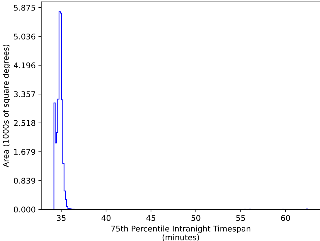
roll_uniform_early_half_mjdp0_v3.4_10yrs All sky: 75th Percentile Intranight Timespan
