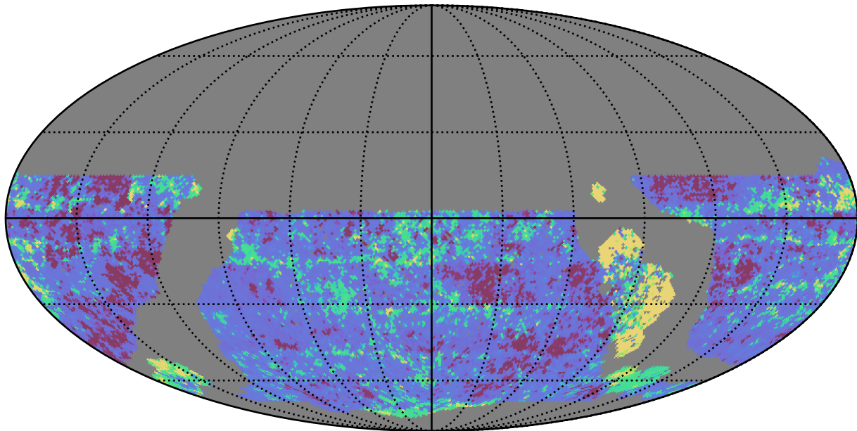
roll_uniform_early_half_mjdp0_v3.4_10yrs WFD y band: 20thPercentile Inter-Night Gap
