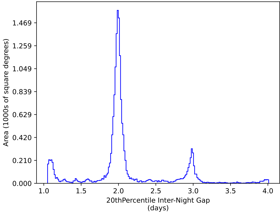
roll_uniform_early_half_mjdp0_v3.4_10yrs WFD y band: 20thPercentile Inter-Night Gap
