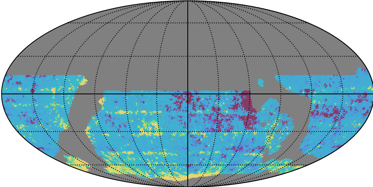
roll_uniform_early_half_mjdp0_v3.4_10yrs WFD r band: 20thPercentile Inter-Night Gap
