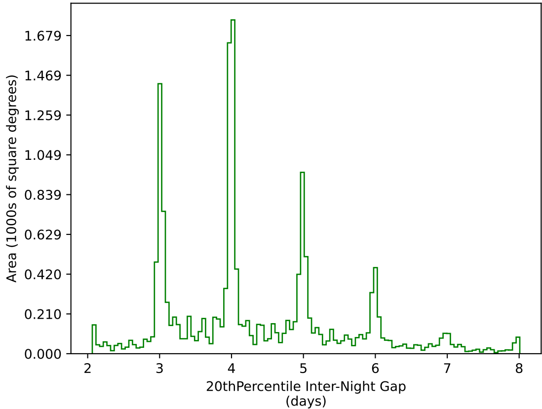
roll_uniform_early_half_mjdp0_v3.4_10yrs WFD g band: 20thPercentile Inter-Night Gap
