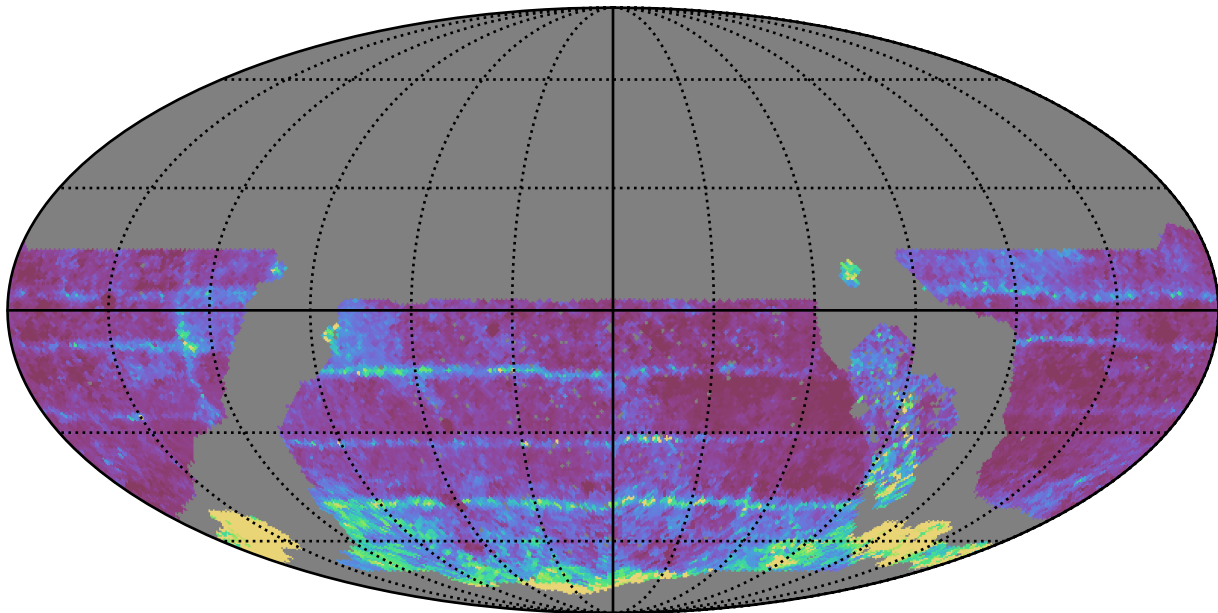
roll_uniform_early_half_mjdp0_v3.4_10yrs WFD all bands: 20thPercentile Inter-Night Gap
