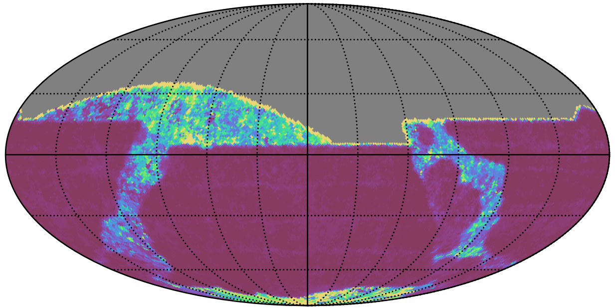
roll_uniform_early_half_mjdp0_v3.4_10yrs All sky z band: 20thPercentile Inter-Night Gap
