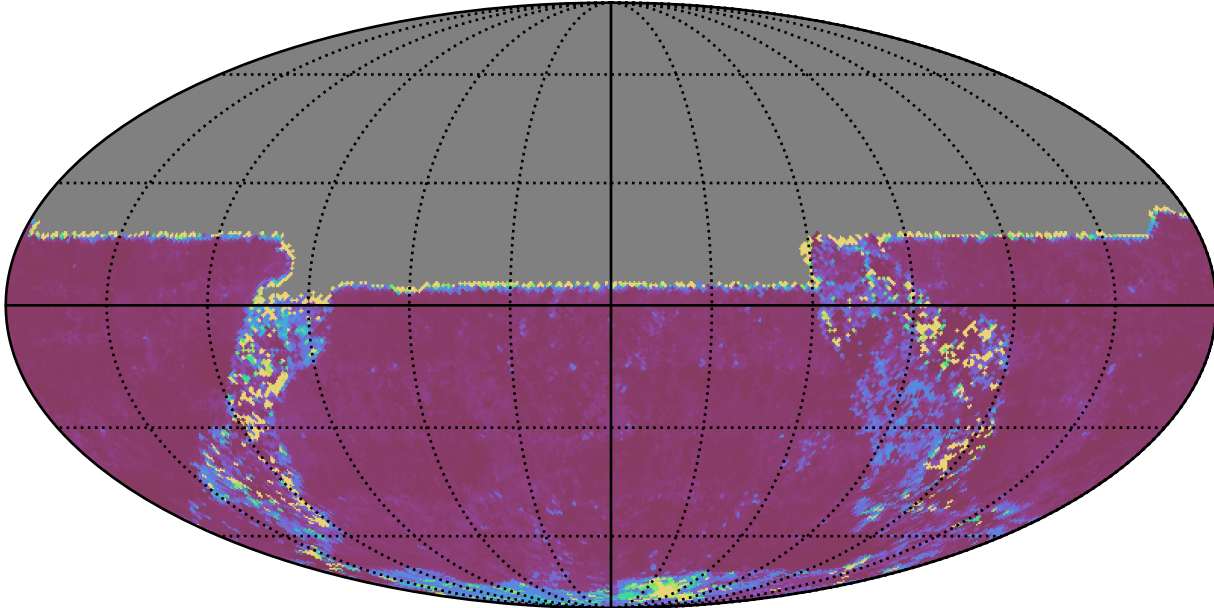
roll_uniform_early_half_mjdp0_v3.4_10yrs All sky u band: 20thPercentile Inter-Night Gap
