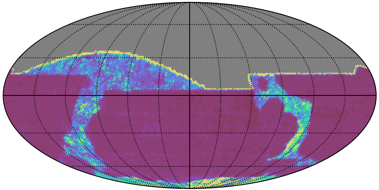
roll_uniform_early_half_mjdp0_v3.4_10yrs All sky r band: 20thPercentile Inter-Night Gap
