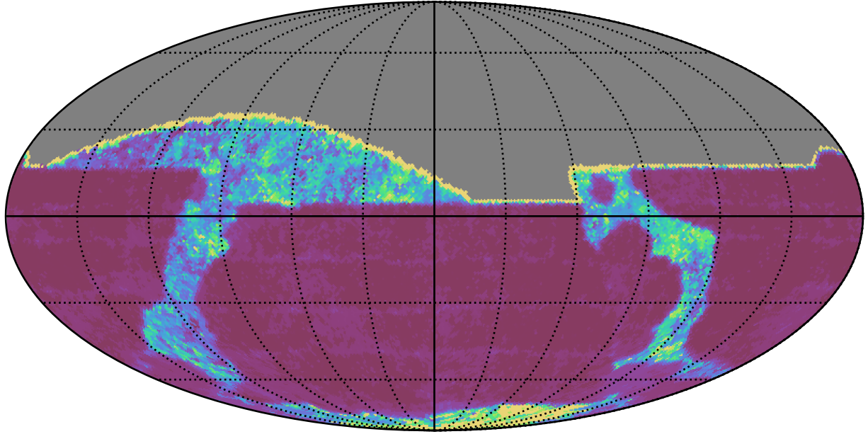
roll_uniform_early_half_mjdp0_v3.4_10yrs All sky i band: 20thPercentile Inter-Night Gap
