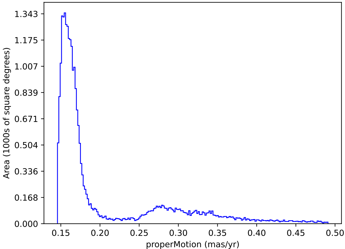
roll_uniform_early_half_mjdp0_v3.4_10yrs : properMotion
