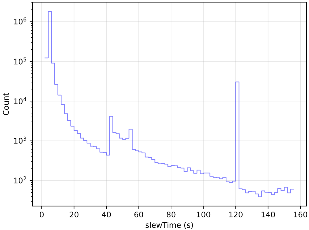
roll_uniform_early_half_mjdp0_v3.4_10yrs All visits: Slew Time Histogram
