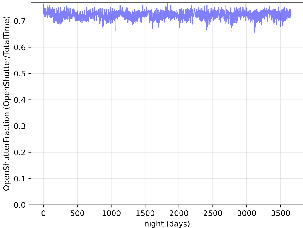
roll_uniform_early_half_mjdp0_v3.4_10yrs : OpenShutterFraction
