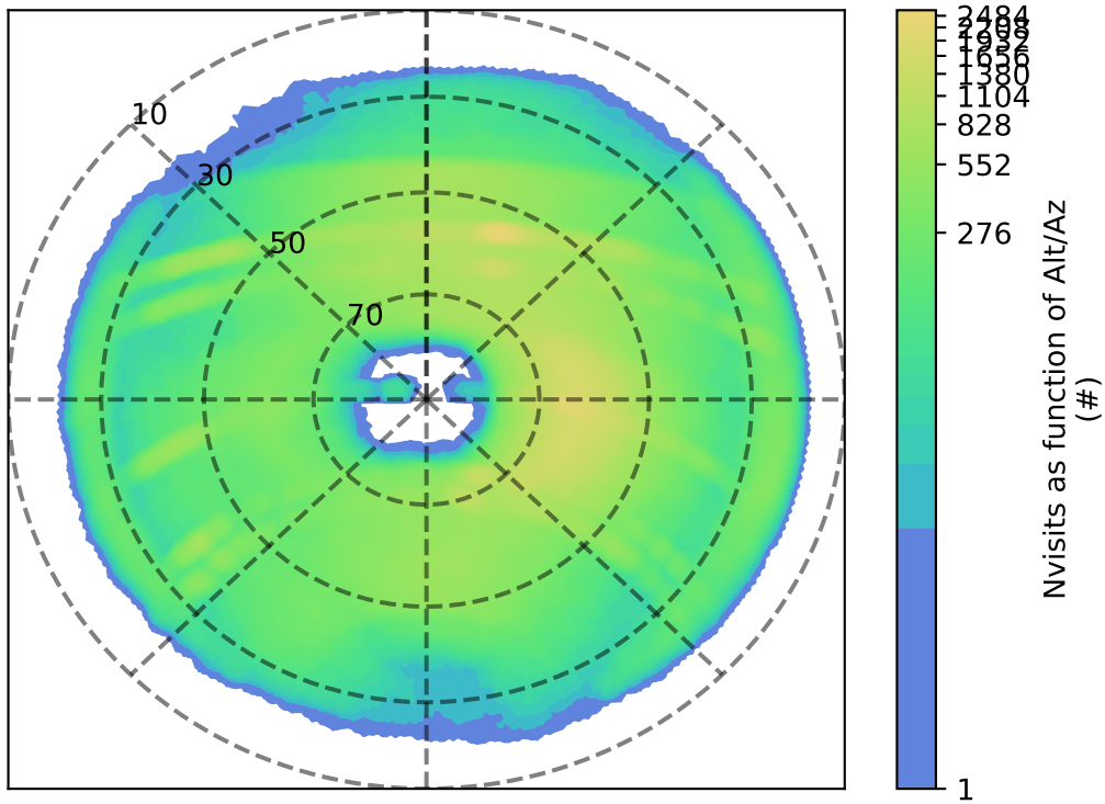
roll_uniform_early_half_mjdp0_v3.4_10yrs z: Nvisits as function of Alt/Az
