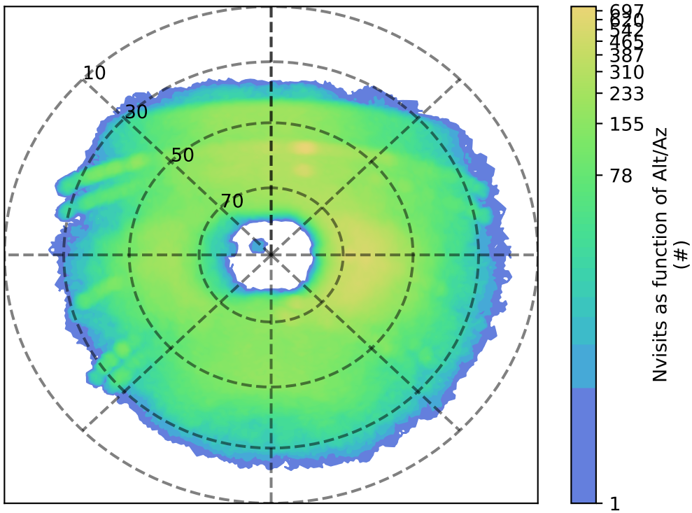
roll_uniform_early_half_mjdp0_v3.4_10yrs u: Nvisits as function of Alt/Az
