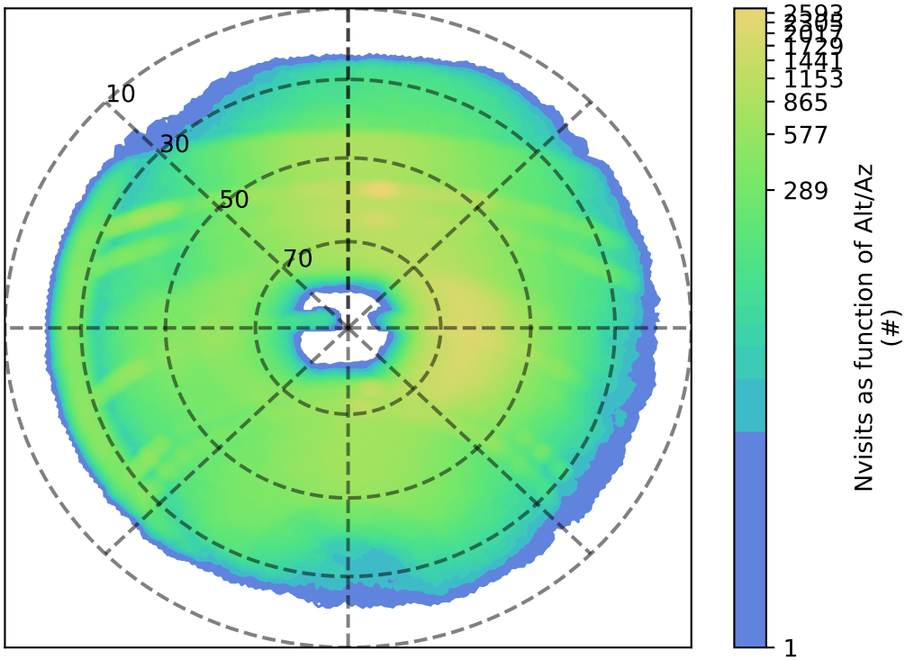
roll_uniform_early_half_mjdp0_v3.4_10yrs r: Nvisits as function of Alt/Az
