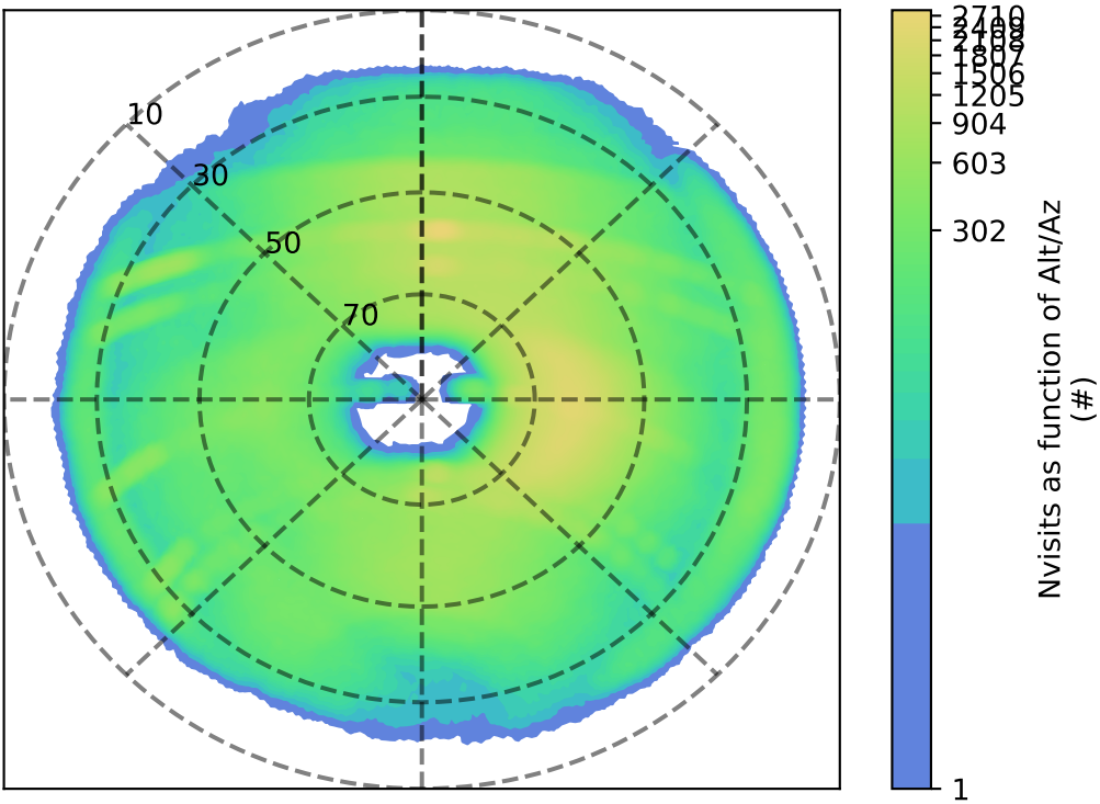
roll_uniform_early_half_mjdp0_v3.4_10yrs i: Nvisits as function of Alt/Az
