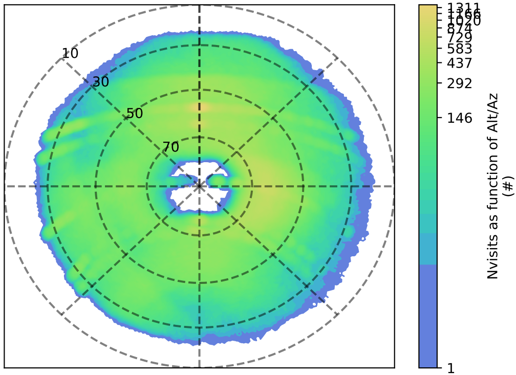
roll_uniform_early_half_mjdp0_v3.4_10yrs g: Nvisits as function of Alt/Az
