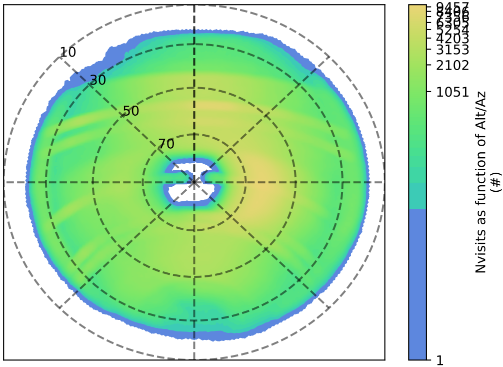
roll_uniform_early_half_mjdp0_v3.4_10yrs : Nvisits as function of Alt/Az
