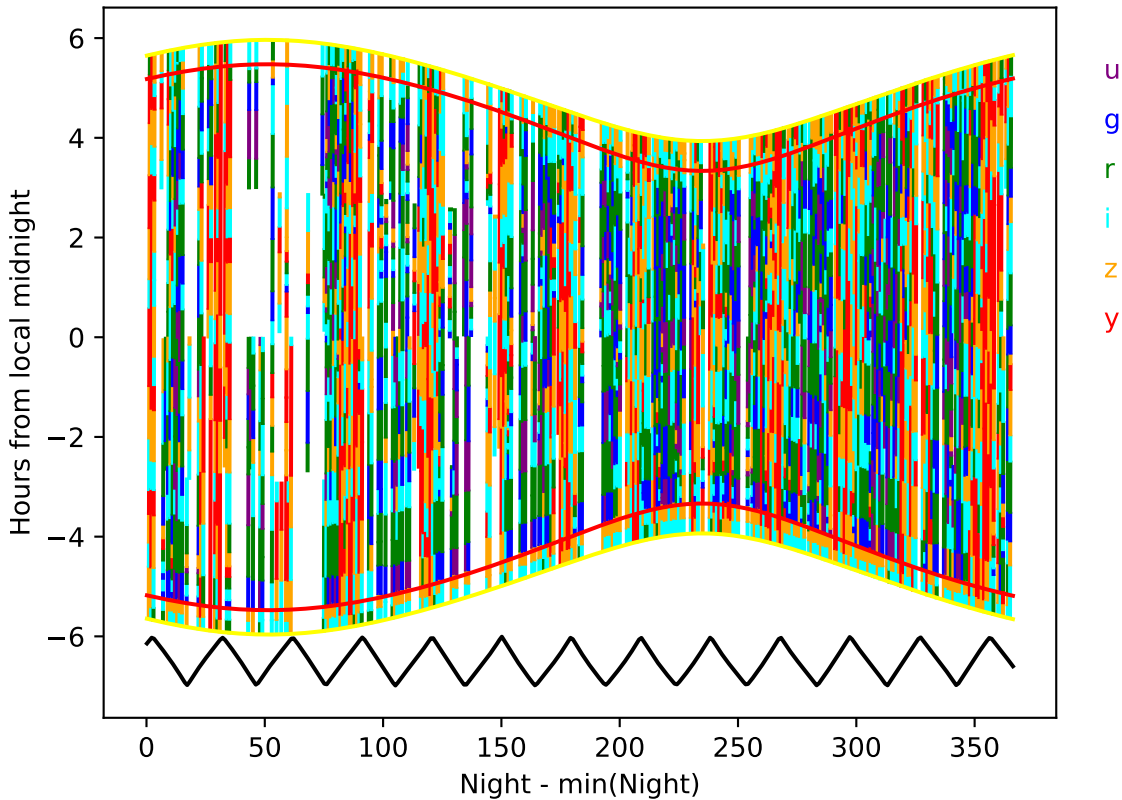
roll_uniform_early_half_mjdp0_v3.4_10yrs year 9-10: Hourglass
