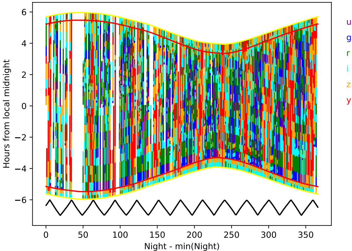
roll_uniform_early_half_mjdp0_v3.4_10yrs year 6-7: Hourglass
