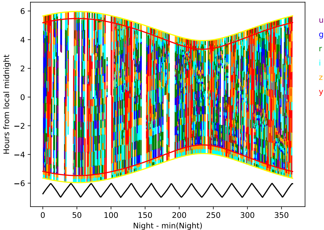
roll_uniform_early_half_mjdp0_v3.4_10yrs year 0-1: Hourglass
