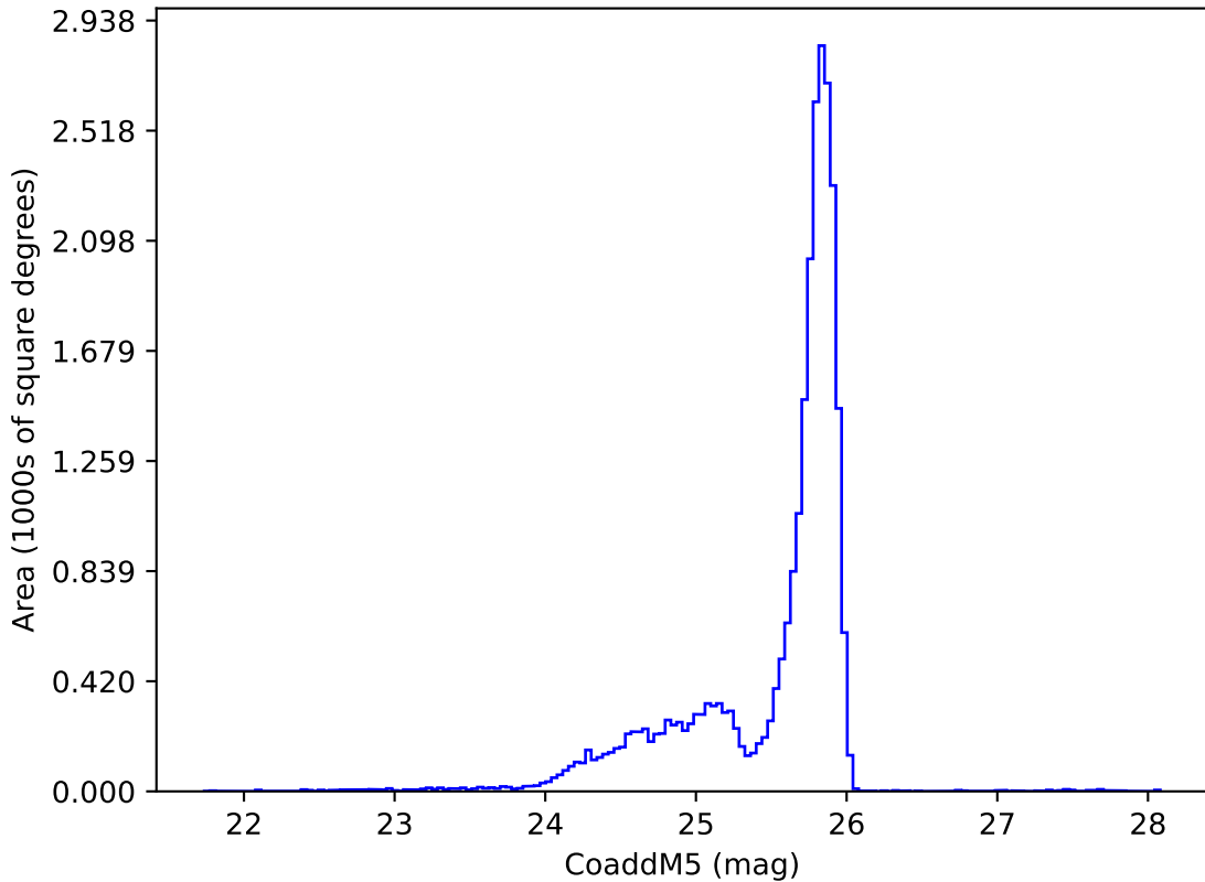
roll_uniform_early_half_mjdp0_v3.4_10yrs z: CoaddM5
