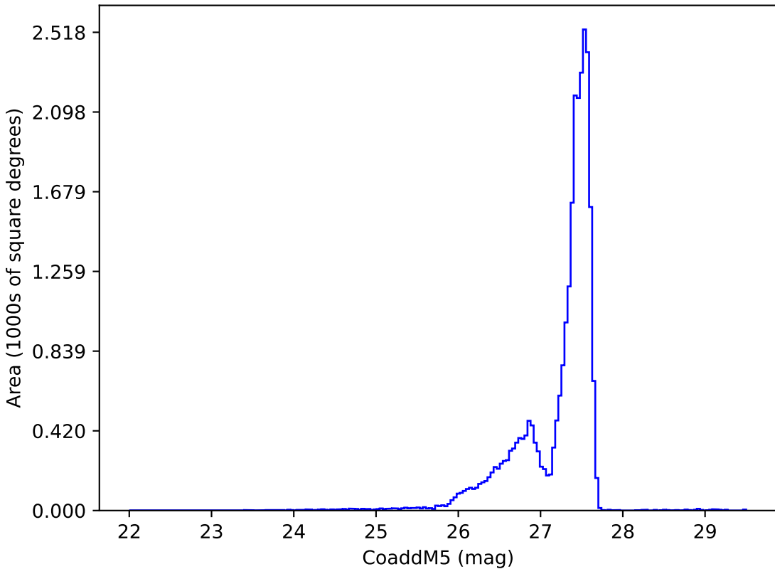
roll_uniform_early_half_mjdp0_v3.4_10yrs : CoaddM5
