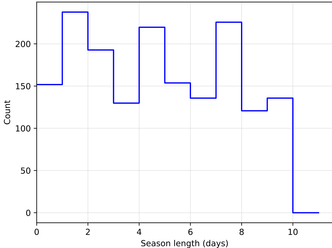
roll_uniform_early_half_mjdp0_v3.4_10yrs DD:WFD all bands: SeasonLength
