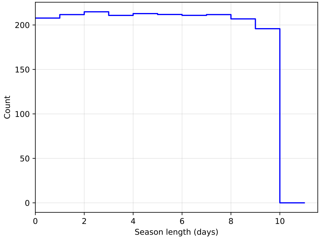
roll_uniform_early_half_mjdp0_v3.4_10yrs DD:EDFS all bands: SeasonLength
