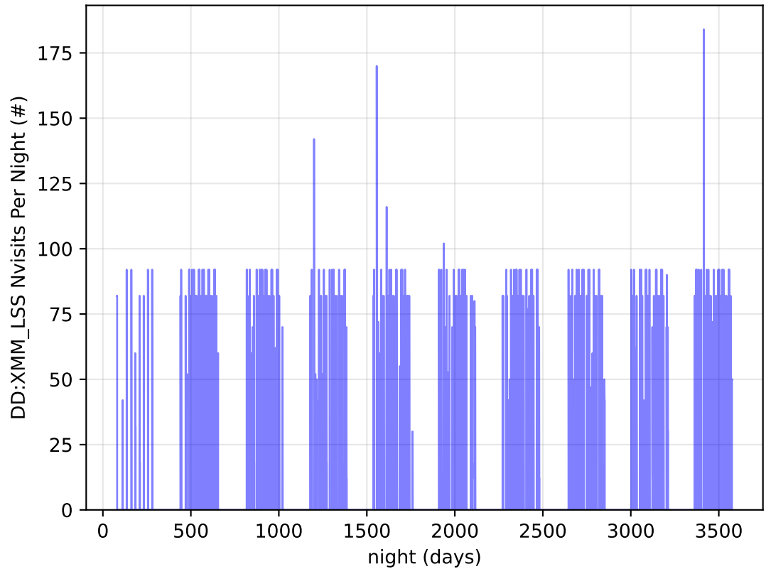
roll_uniform_early_half_mjdp0_v3.4_10yrs all bands: DD:XMM_LSS Nvisits Per Night
