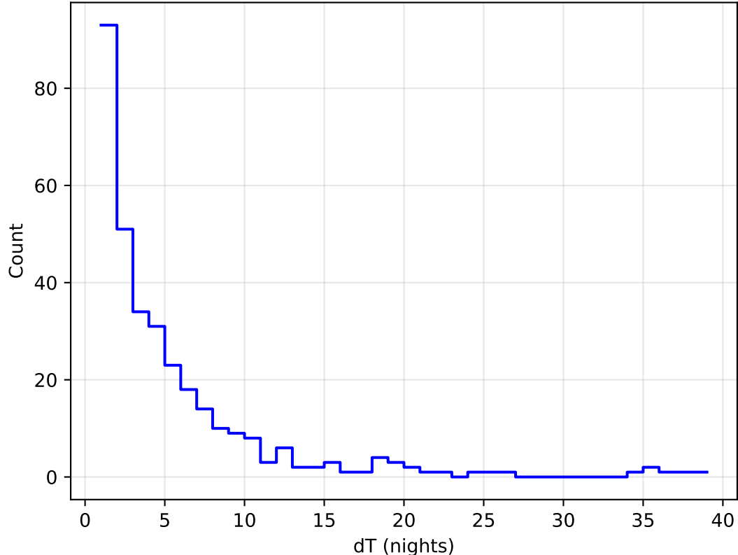
roll_uniform_early_half_mjdp0_v3.4_10yrs all bands: DD:WFD Delta Nights Histogram
