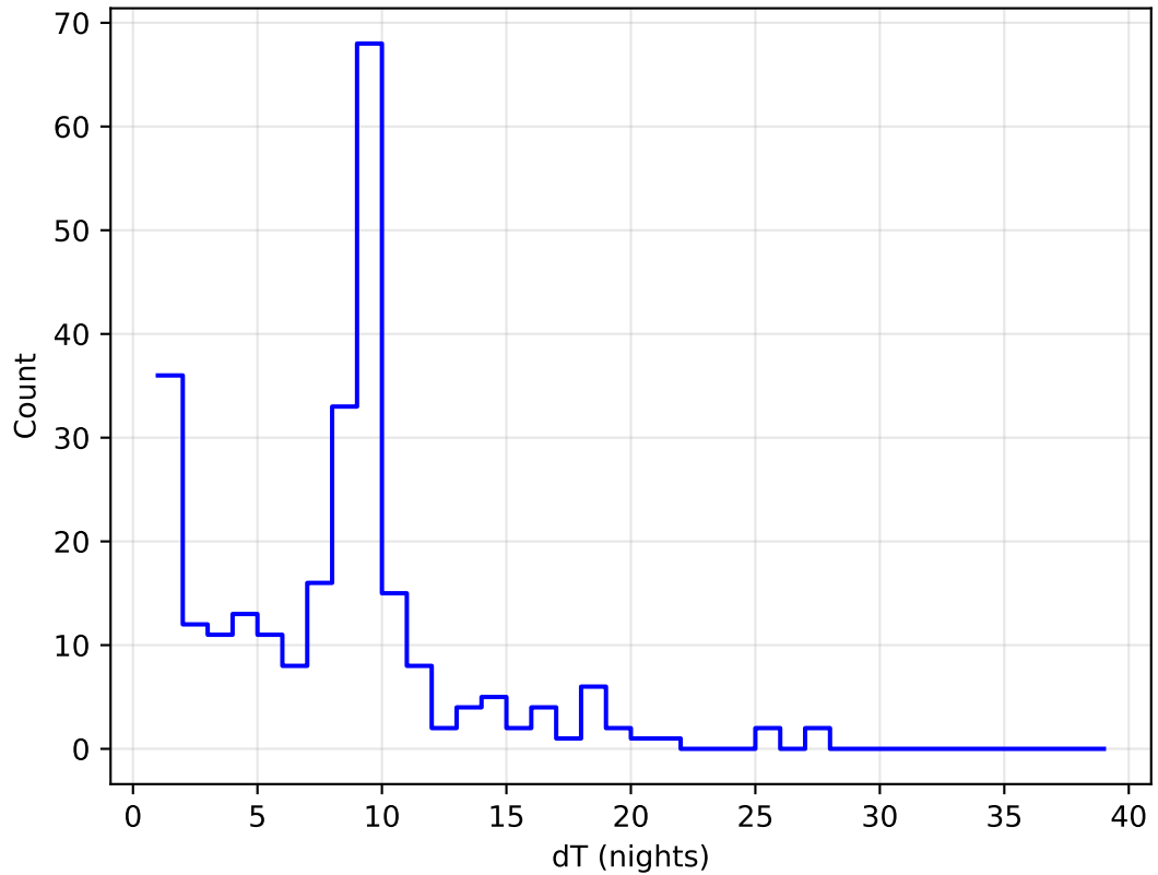
roll_uniform_early_half_mjdp0_v3.4_10yrs all bands: DD:ELAISS1 Delta Nights Histogram
