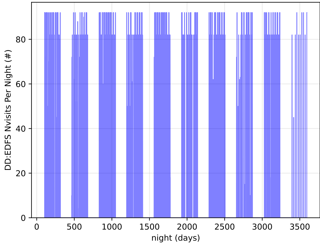
roll_uniform_early_half_mjdp0_v3.4_10yrs all bands: DD:EDFS Nvisits Per Night
